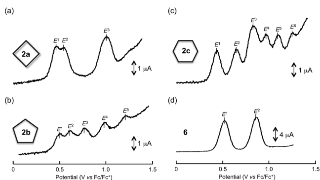
Figure 3. DPV charts for a) 2a , b) 2b , c) 2c , and d) 6 .
